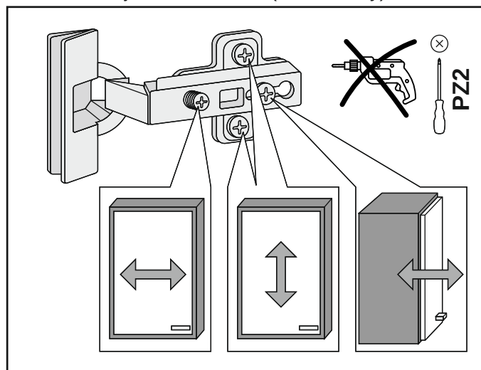
Türverstellschema (falls esforderlich) Door adjustment scheme (if necessary)
