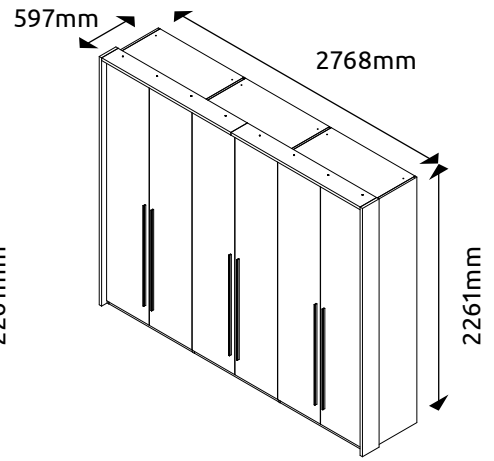
P6B/PN LWH - 2768x597x2261
