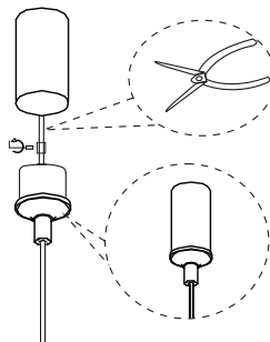
8. Adjust the wire & fix it into place
