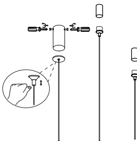
7. Apply side screws and make Hanging elements stable
