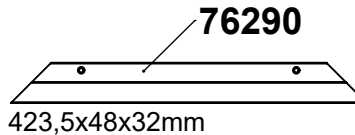
423,5x48x32mm
