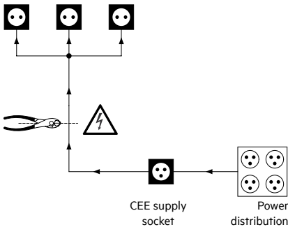
230 V sockets in caravan/recreational vehicle
