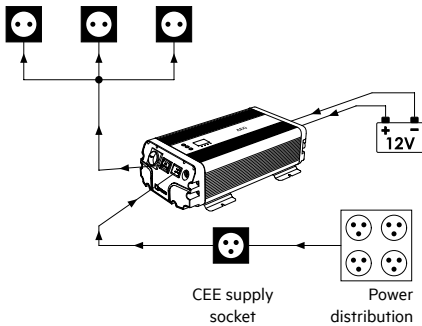
230 V sockets in caravan/recreational vehicle
