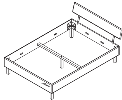
ITM: 415712+415713 BxHxT: 145,2x42x205,2+ 145,2x2,1x24cm
