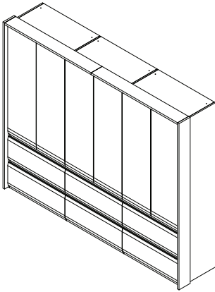
P66/IC LWH - 2768x597x2261
